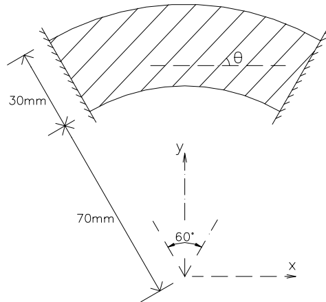
Figure 1. Aluminum metal-matrix composite arch beam.
