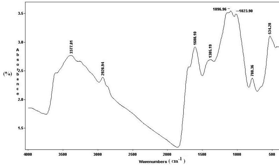
Figure 1b. FT.i.r. spectra of Seyiömer lignite which oxidized by air
