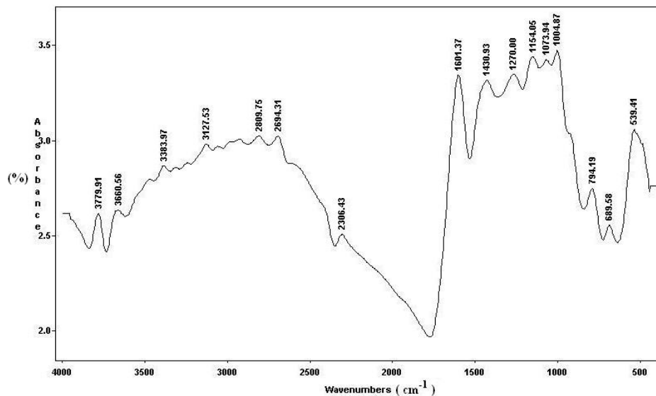
Figure 2a. FT.i.r. spectra of original Tunçbilek lignit
