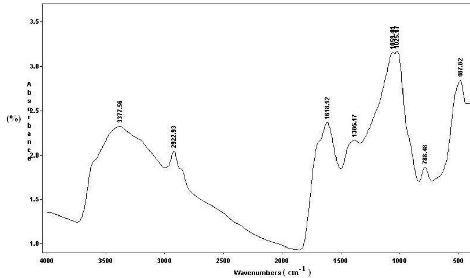
Figure 1c. FT.i.r. spectra of Seyitömer lignite which oxidized by H 2 O 2 solution
