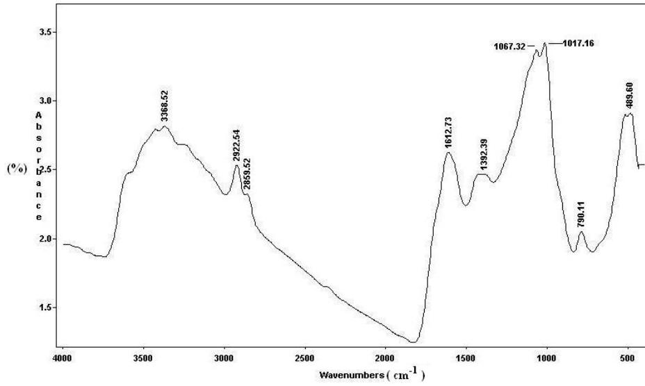
Figure 1a. FT.i.r. spectra of original Seyiömer lignite
