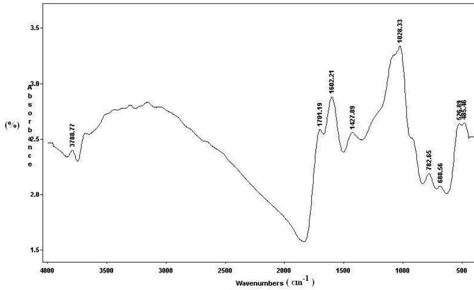
Figure 2b. FT.i.r. spectra of Tunçbilek lignite which oxidized by air
